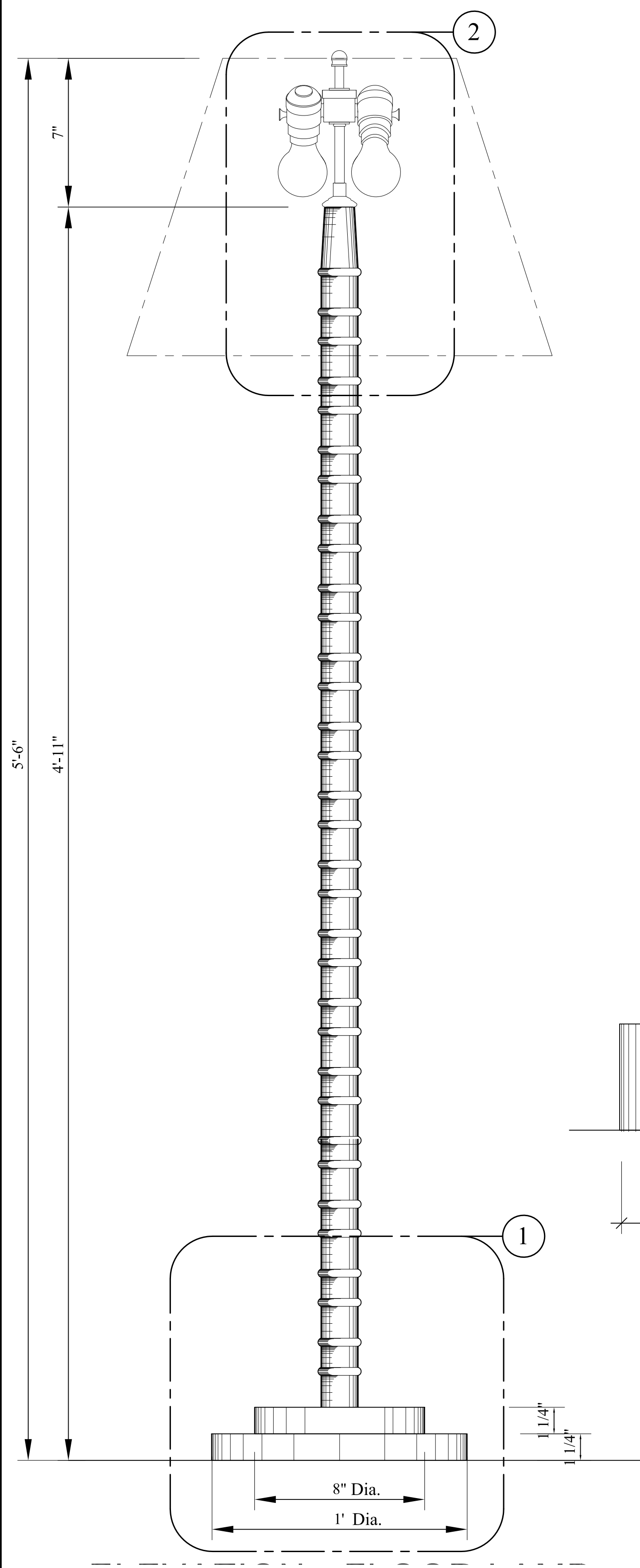
ELEVATION - FLOOR LAMP 3
