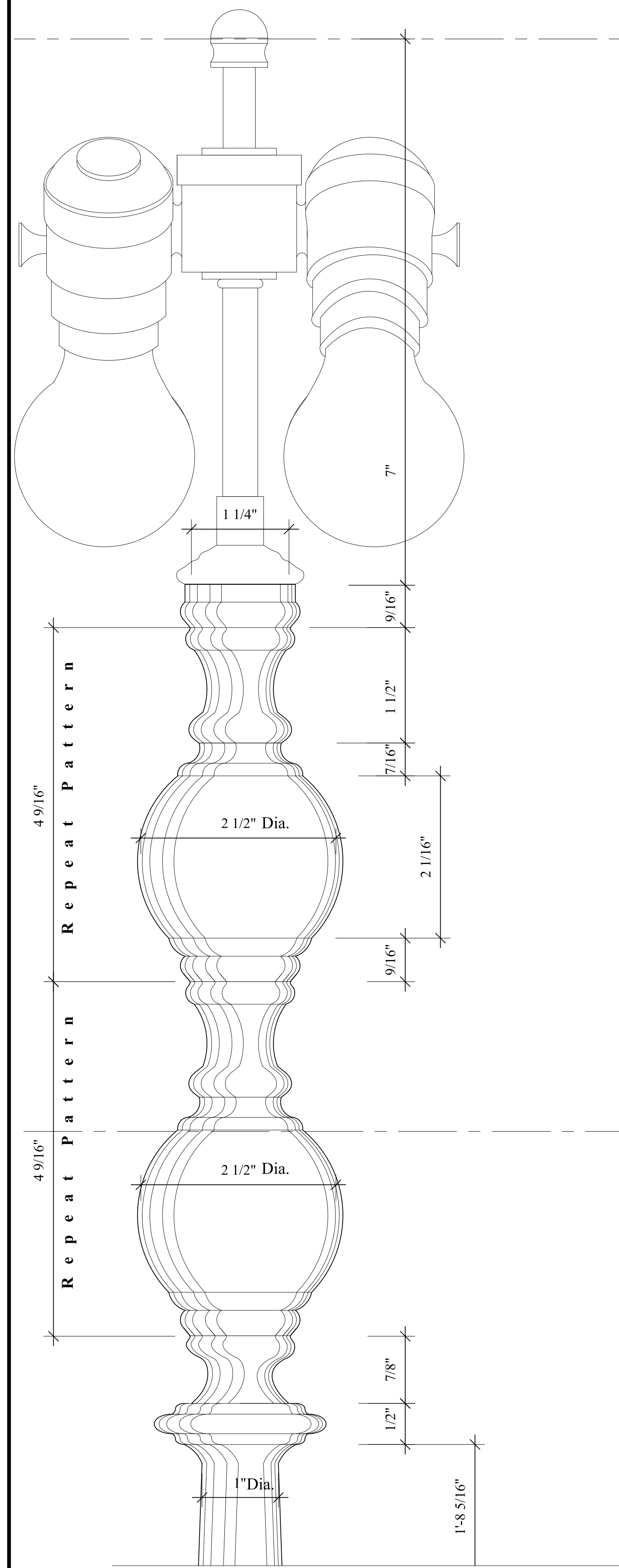
SPOT DETAIL 1 - FLOOR LAMP SCALE: FULL SCALE
