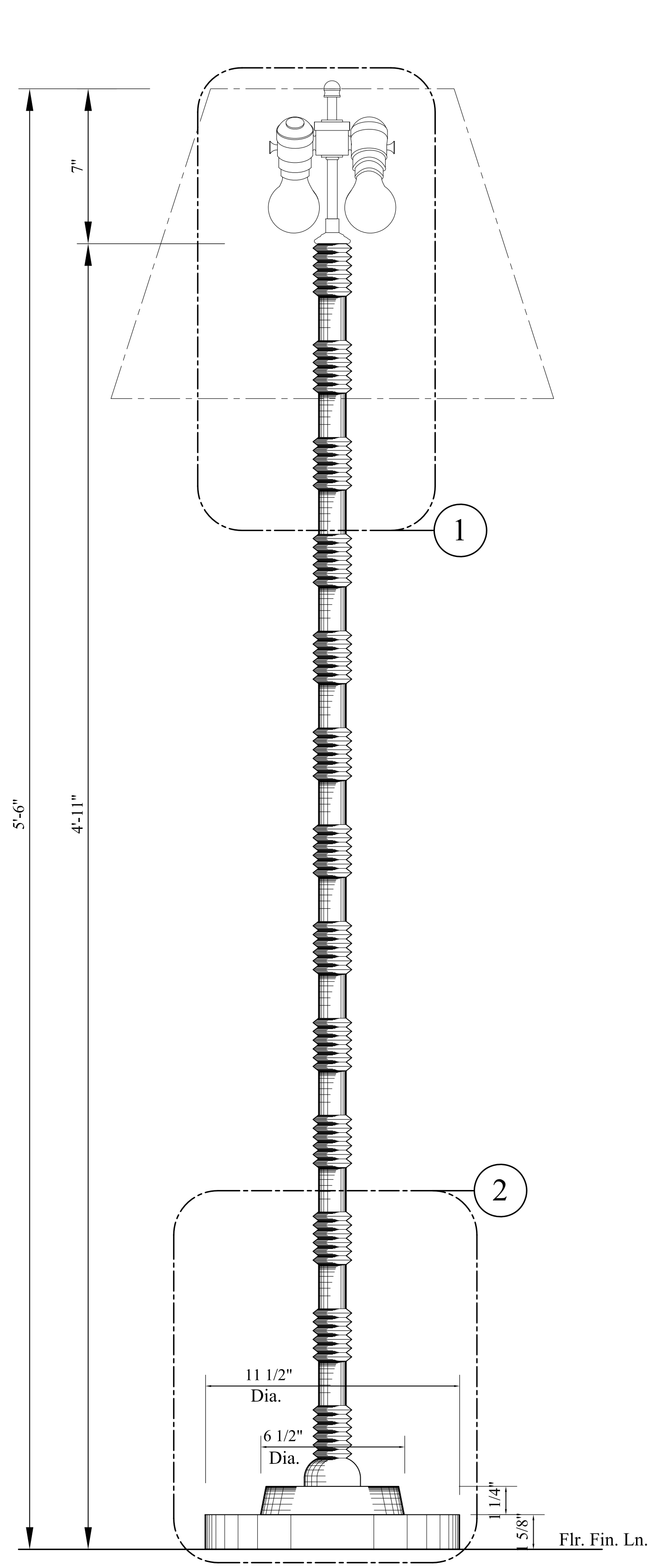
ELEVATION - FLOOR LAMP 1 SCALE : 3" = 1'-0"
